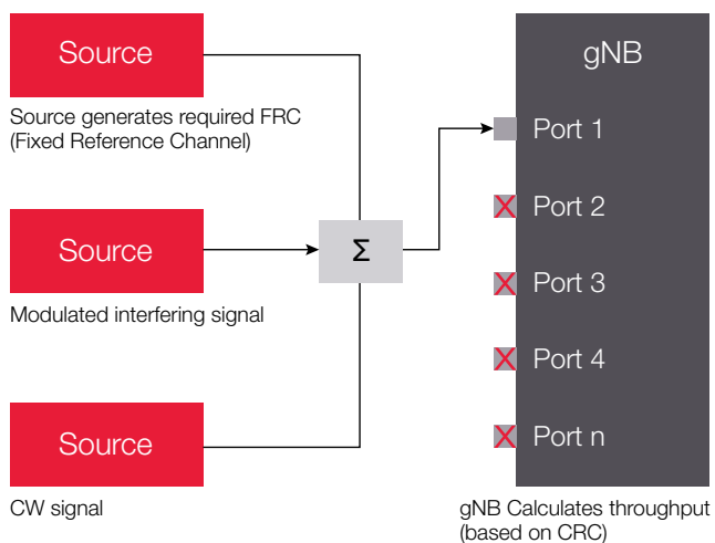
Figure 9.1. Base station receiver intermodulation conducted test setup for part 1 (part 2 is OTA)
