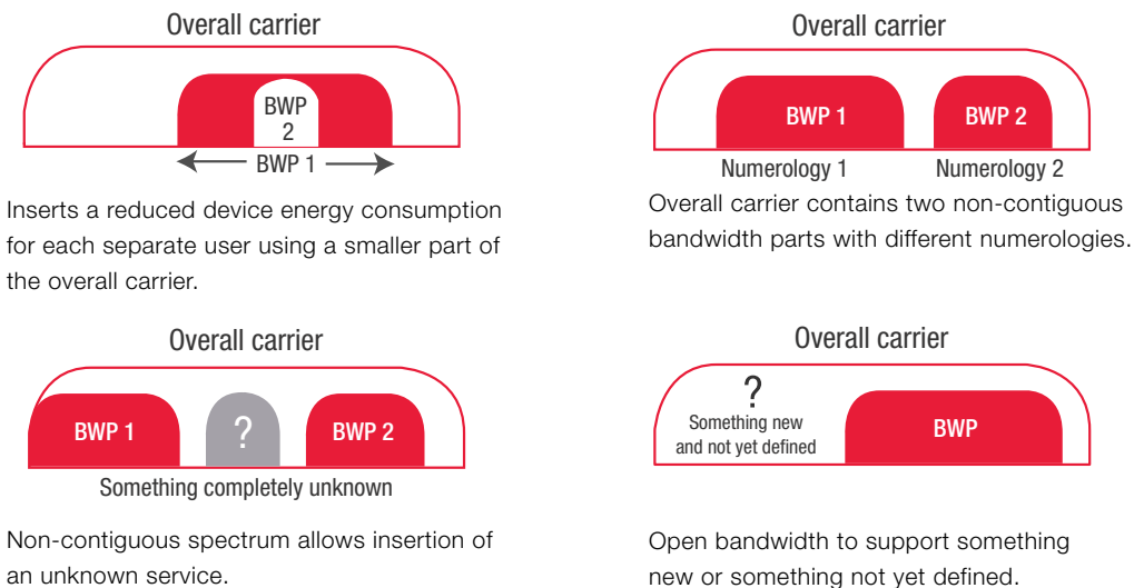
Figure 2.5. Bandwidth parts support multiplexing of different services on the same carrier
