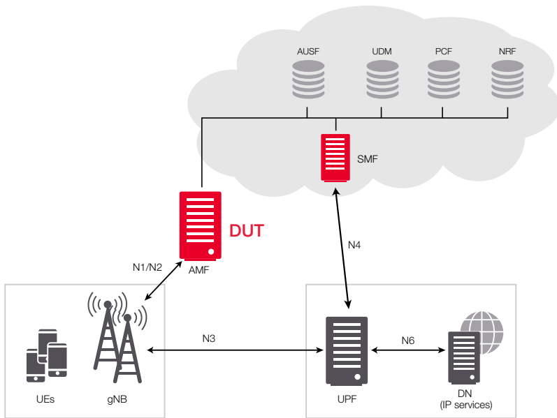
Figure 23.3. AMF isolation use case
