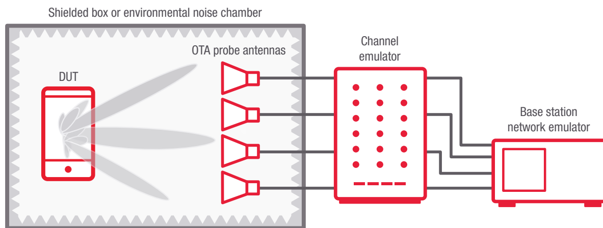
Figure 5.7. A base station emulator and channel emulator simulate real-world conditions
