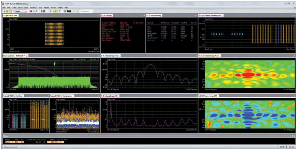
Figure 3.3. Analysis of a 5G NR 256 QAM signal with antenna pattern
